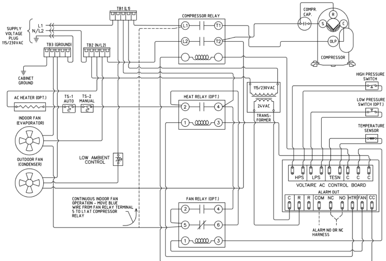
Figure 3 – AN02 / AS02 Electrical Wiring Diagram (No Hard Start)
